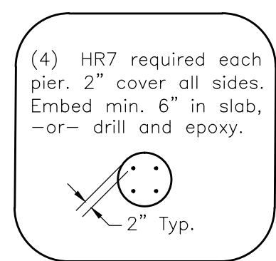
SAFETY PIER REINFORCING Top View
